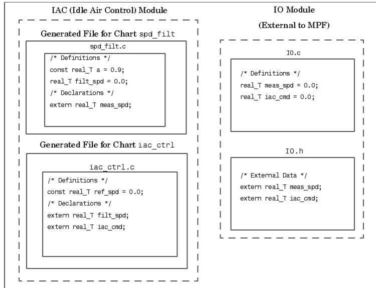
Engine Idle Speed Control System (Ownership Example)
